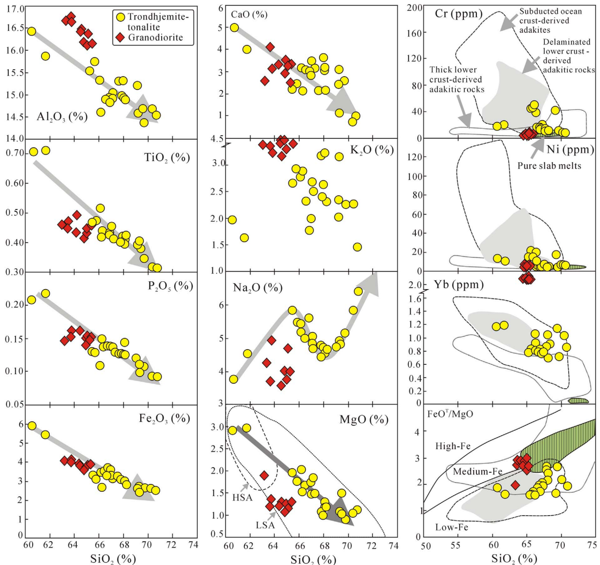
Fig. 9. Harker diagrams of the Neoproterozoic granitic intrusions in Mazar terrane (three samples reported by (Bian et al., 2013) was also included, HAS-high \text{SiO}_2 adakite, LSA-low \text{SiO}_2 adakite, the ranges of the HSA and LSA are from (Martin et al., 2005) and the ranges of the variable types of adakitic rocks are from Wang et al., 2006. See more details in the text).
