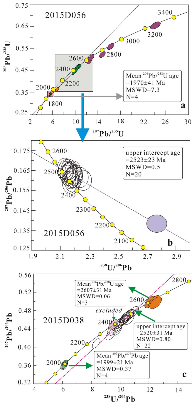
Fig. 5. Concordia of the zircon U-Pb ages of the meta -rhyolite from the Archaean basement of the Mazar terrane (see details in the text).
