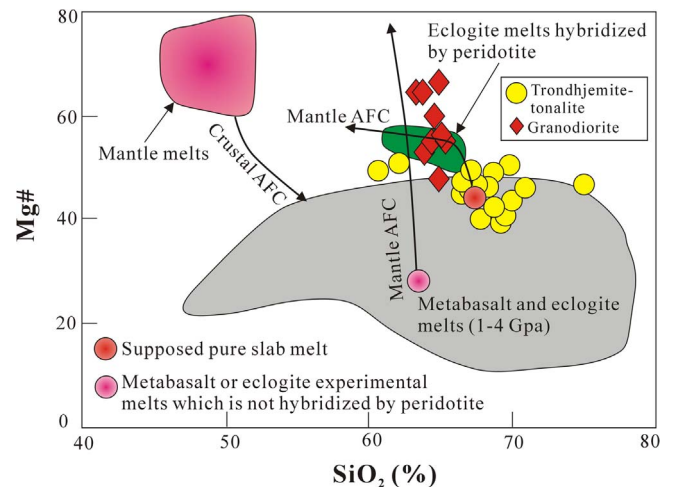
Fig. 14. \text{SiO}_2 vs. Mg# diagram. The mantle/crustal AFC curves are after Stern and Kilian (1996) (curves 1 and 3) and Rapp et al. (1999) (curve 2). The starting points of curves 1 and 2 represent a pure slab-melt composition and metabasaltic or eclogite experimental melt (Stern and Kilian, 1996) (Rapp et al., 1999), respectively. The field of metabasaltic and eclogite melts (1–4.0 GPa) is after Stern and Kilian (1996). The fields of metabasaltic and eclogite experimental melts that are hybridized with peridotite are after Rapp et al. (1999).
