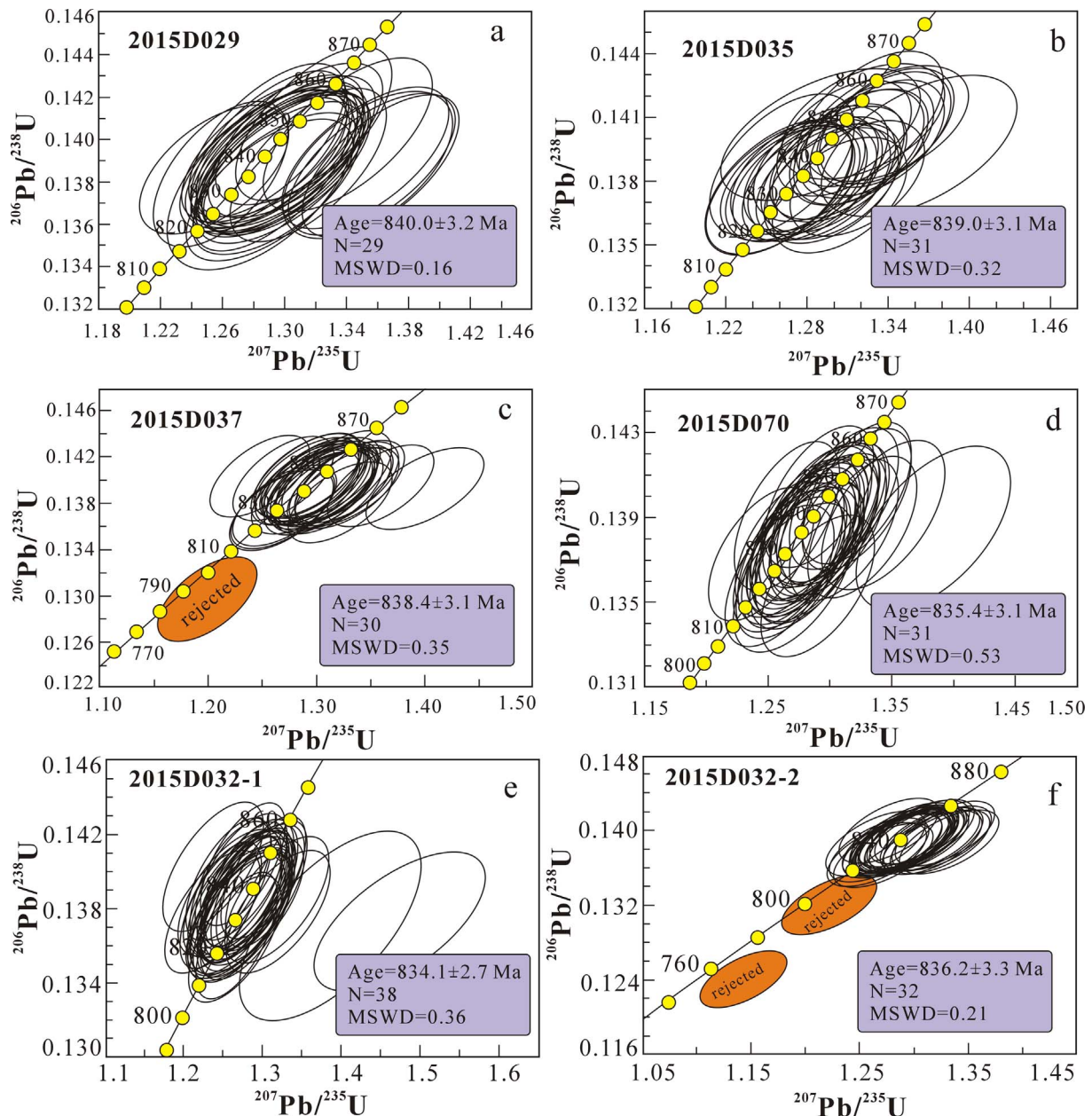
Fig. 6. Concordia of the zircon U-Pb data of the Neoproterozoic granitic intrusions in the Mazar terrane (see details in the text).
