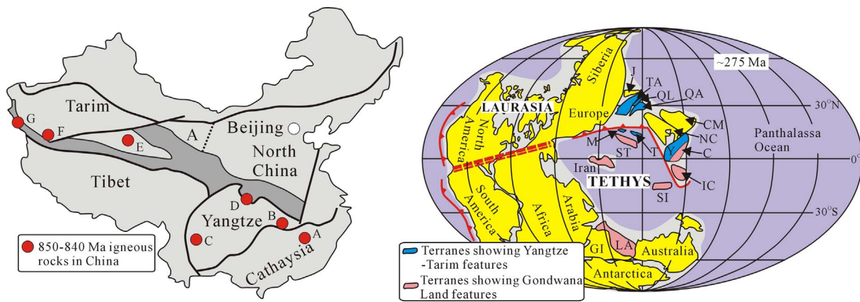
Fig. 15. (a) Distribution of the 850–840 Ma igneous activities in China: A: the bimodal volcanic sequence in Cathaysia (Li et al., 2008b); B: ~850 Ma Shenu diorite in Yangtze (Li et al., 2008c); C: ~850 Ma Guandaoshan granodiorite in western Yangtze (Li et al., 2003b); D: ~850 Ma diorite at the northern margin of the Yangtze Block (Wang et al., 2012); E: ~850 Ma high-Ti and low-Ti CFB in Qaidam terrane (Song et al., 2010); F: 850–830 Ma OIB-like basalt in SW Tarim (Zhang et al., 2016); G: 840–835 Ma trondhjemite-tonalites and granodiorites (this study); (b) Two types of terranes distributed in Tibet Plateau, i.e., the Tarim–Yangtze affinity type and the Gondwana affinity type. J–Junggar, TA–Tarim, QL–Qilian, QA–Qaidam, NC–North China, T–Tianshuihai, M–Mazar, CM–Central Mongolia, ST–Southern Qiangtang, Y–Yangtze, C–Cathaysia, IC–Indochina, SI–Sibumasu (modified after Metcalfe, 2013).
